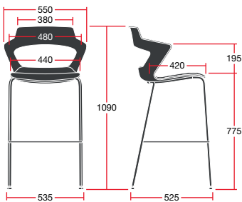
ZENSTUS: Overall Dimensions: 550w x 530d x 1090h
