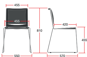
VICM: Overall Dimensions: 550w x 570d x 810h
