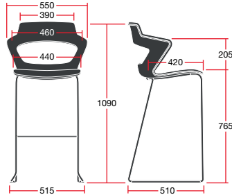
ZENSTSBUSUB: Overall Dimensions: 550w x 520d x 1090h
