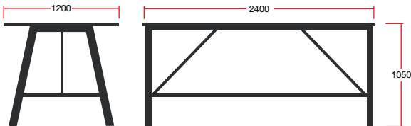
AB24/12: Overall Dimensions: 2400w x 1200d x 1050h
