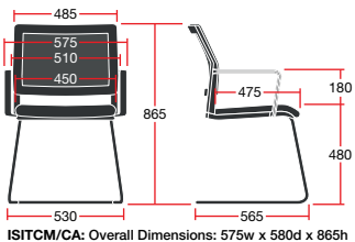
ISITCM/CA: Overall Dimensions: 575w x 580d x 865h
