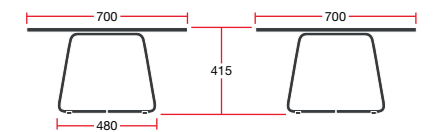
ESCCCT: Overall Dimensions: 700w x 700d x 415h
