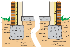
unsuspended subfloor
