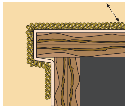
without tread nosing section
