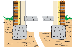
suspended, unventilated subfloor
